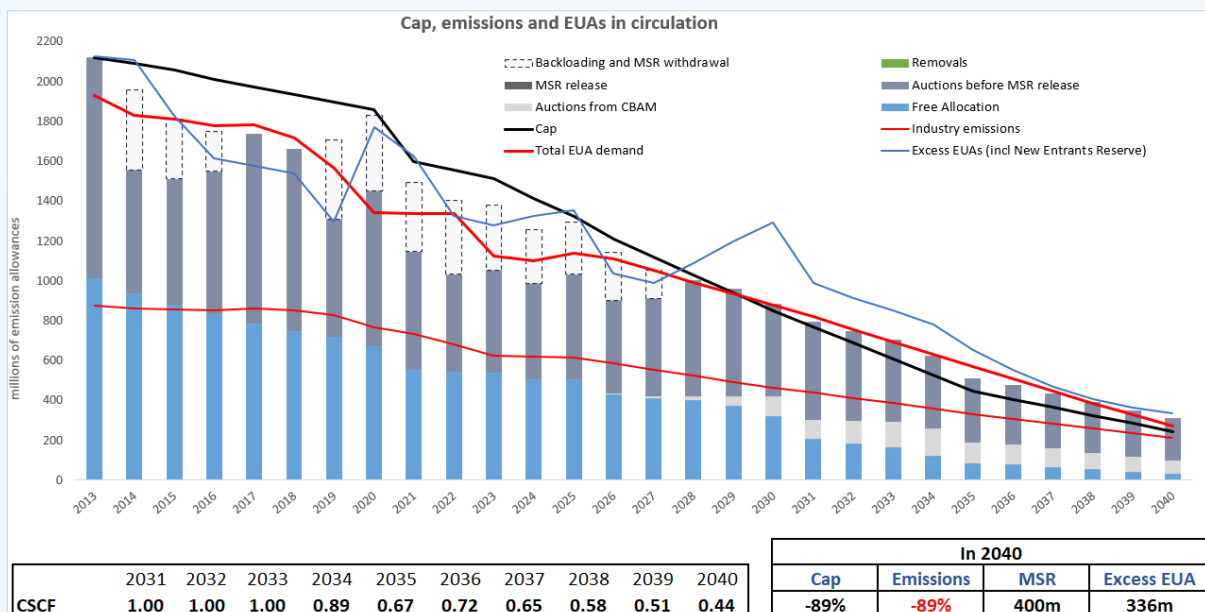
Figure 1: Supply and demand for EUAs in scenario S2, under the Commission's proposed cap (Source: Sandbag's EU ETS Simulator)
